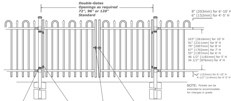
2-1/2" Sq Post-Collar c/w 1/2 Dia x 4" Hinge Bolt 1-1/4" Sq Frame-Collar 1-1/4" Sq Gravity-Catch (lockable) 1-1/4" Sq Finger-Latch Precision Punched Full Tube For Picket Insertion
